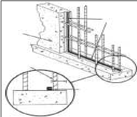
Typical placement of Bentonite Cast Seal at concrete construction joints
